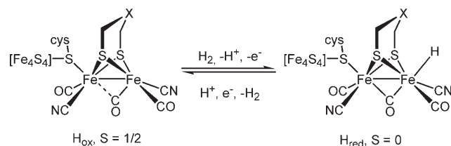
Scheme 1. Two functional states of the active site of the [FeFe] hydrogenases.
